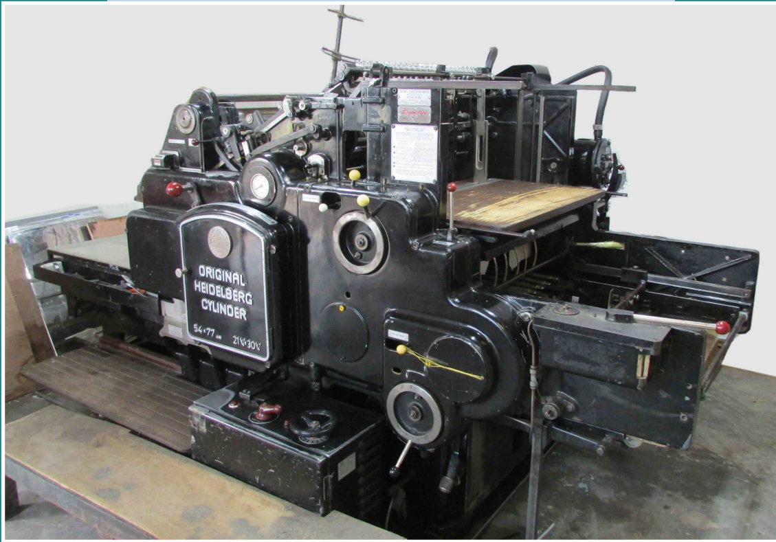
AUTO DIE CUTTING MACHINE
